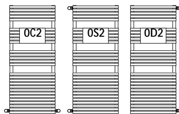
Interaxis (Pipe centre) L=L+13,8 cm Interaxis (Pipe centre) L=H-7,0 cm Interaxis (Pipe centre) L=H-7,0 cm
